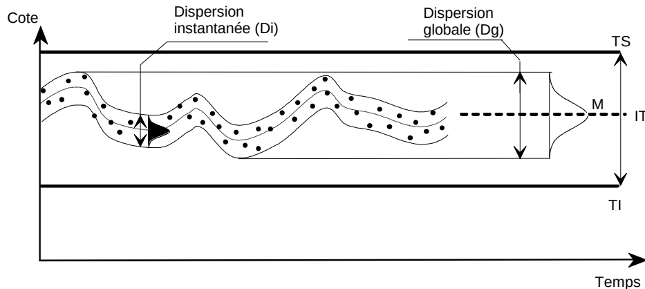
figure 1 – Film de la production
